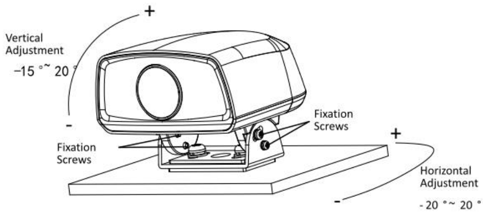
Figure 2-29 Adjusting Angle
