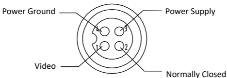
Figure 2-2 Interfaces of Aviation Plug
