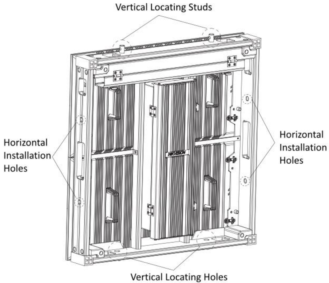
Figure 2-4 Cabinet Frame Locating
