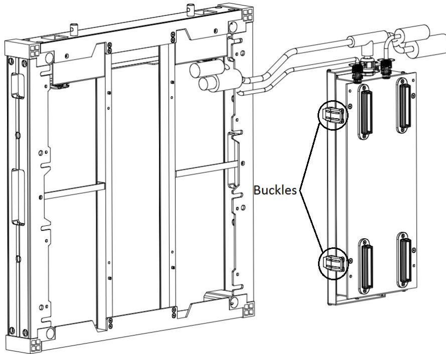
Figure 2-20 Maintain Power Supply Box
