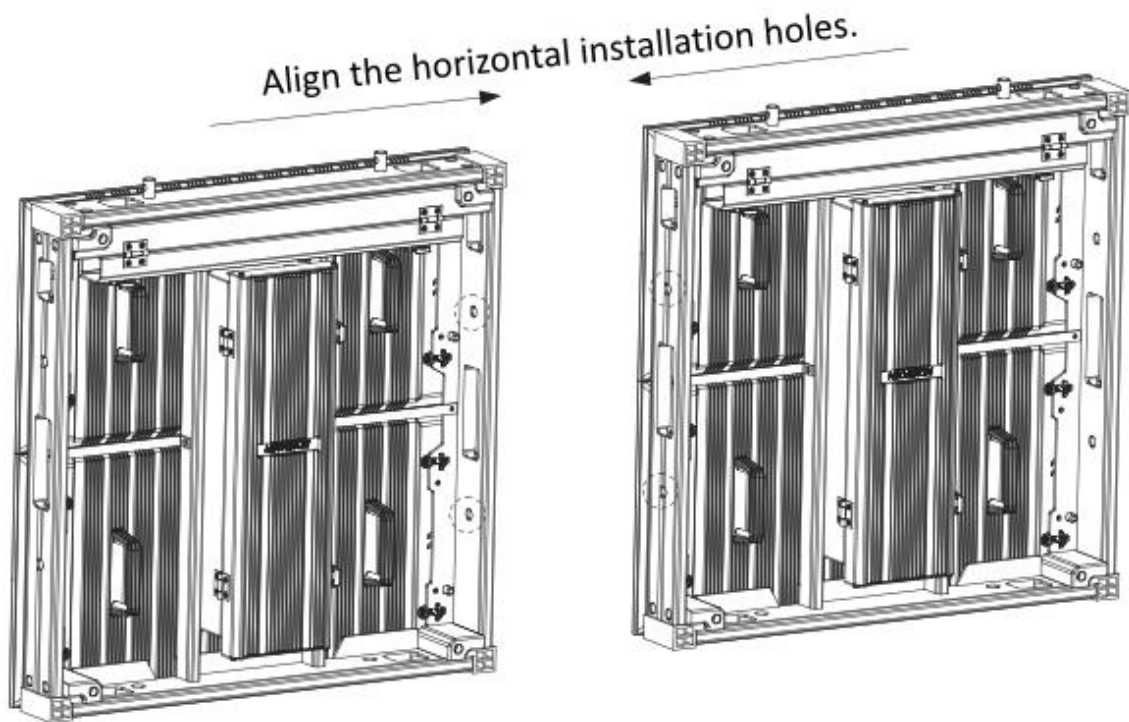
Figure 2-5 Stitch Cabinet Frames Horizontally
