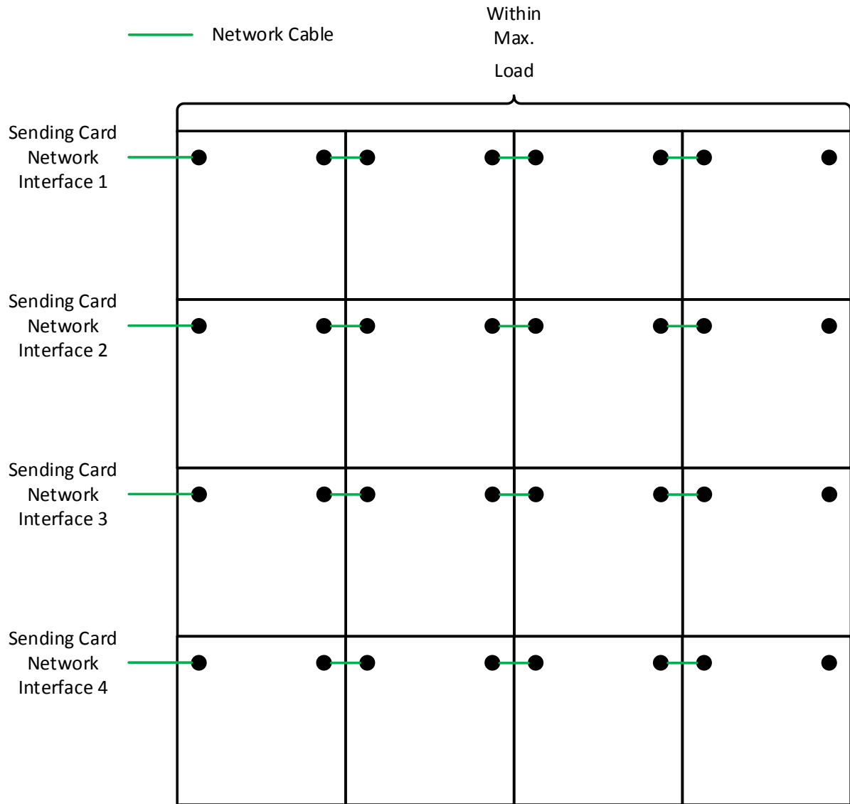
Figure 2-13 Network Cable Connection (Within Max. Load)
