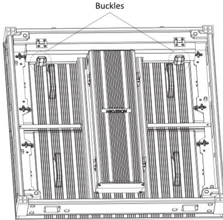
Figure 2-8 Open Wire Hidden Box
