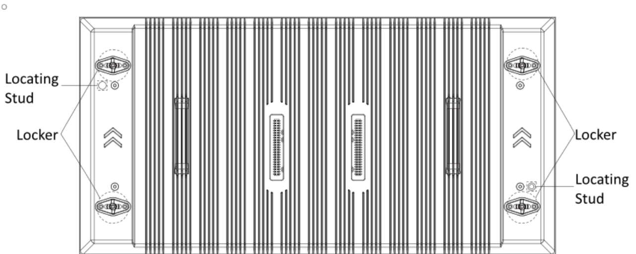
Figure 2-16 Lamp Board Rear View
