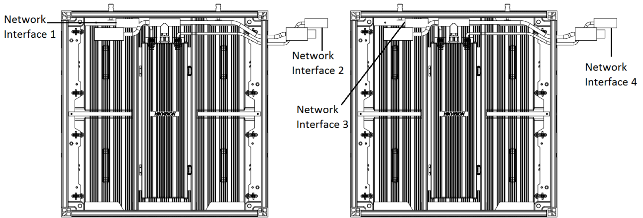
Figure 2-12 Connect Network Cable
