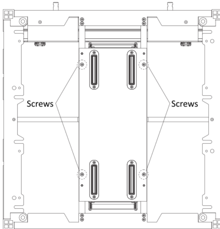
Figure 2-19 Disassemble Power Supply Box
