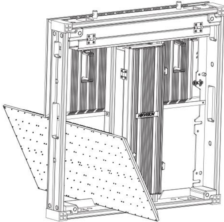
Figure 2-18 Remove Lamp Board
