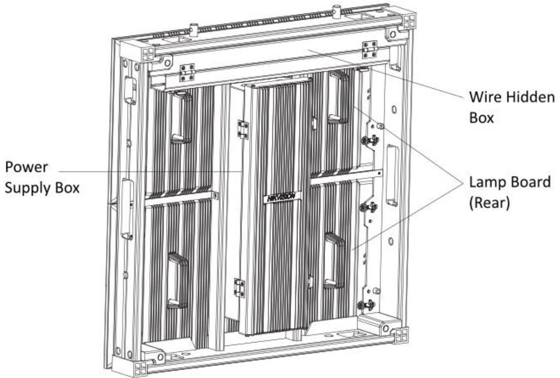
Figure 2-1 Cabinet Overview (Rear)
