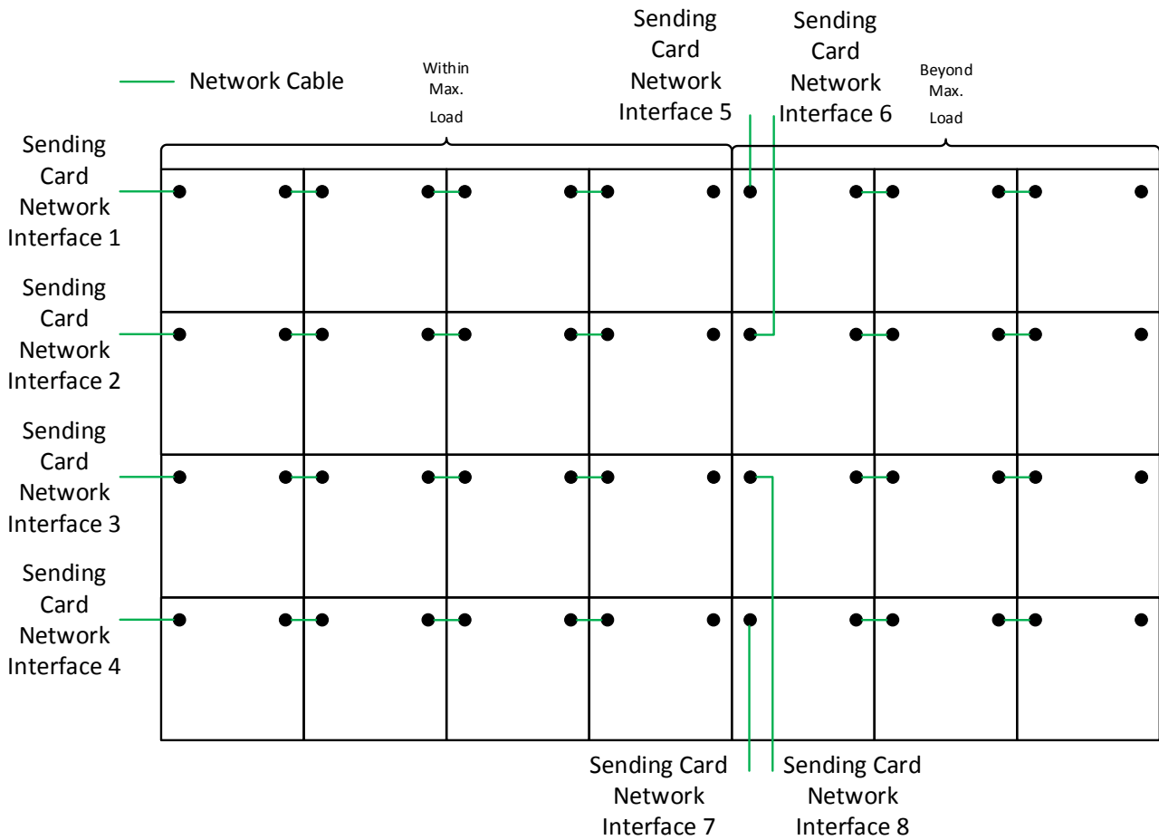
Figure 2-14 Network Cable Connection (Beyond Max. Load)
