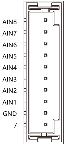
Alarm Input Terminal
