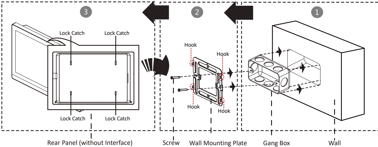
Rear Panel (without Interface)
