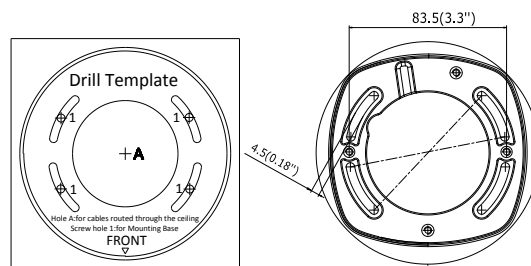
Figure 1-4 Drill Templates and Adapter Plate
