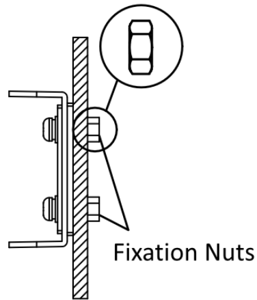
Figure 1-28 Fixation Nuts
