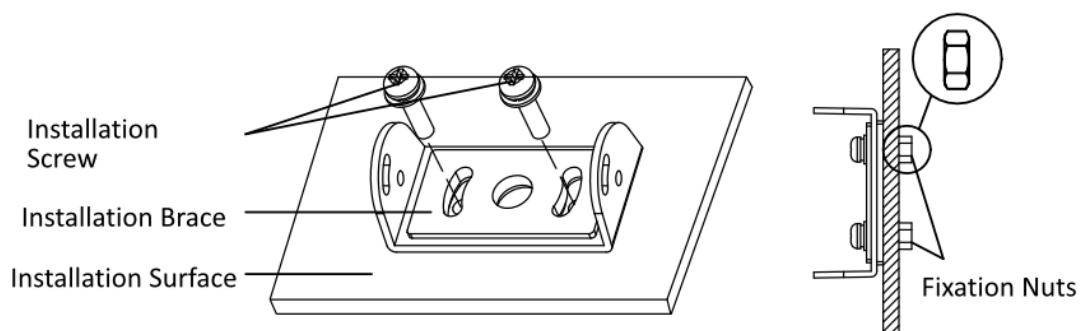
Figure 1-27 Installing Support
