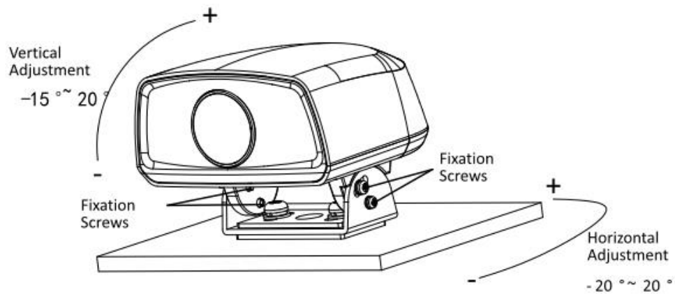
Figure 1-29 Adjusting Angle
