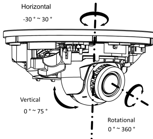
Figure 1-21 Adjusting Angle
