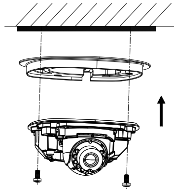
Figure 1-10 Fixed Base
