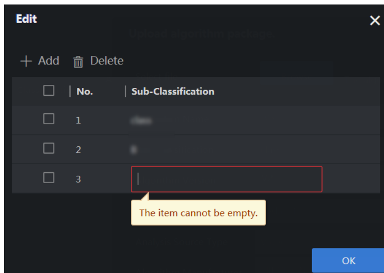
Figure 3-17 Add Sub-Classification
