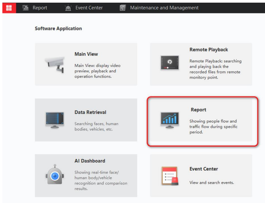
Figure 6-16 Data Report
