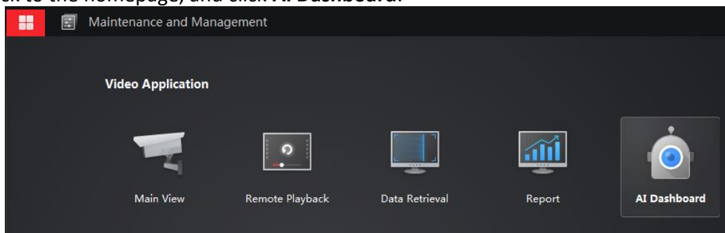
Figure 3-25 AI Dashboard
