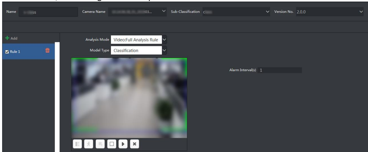
Figure 3-21 Create Task
