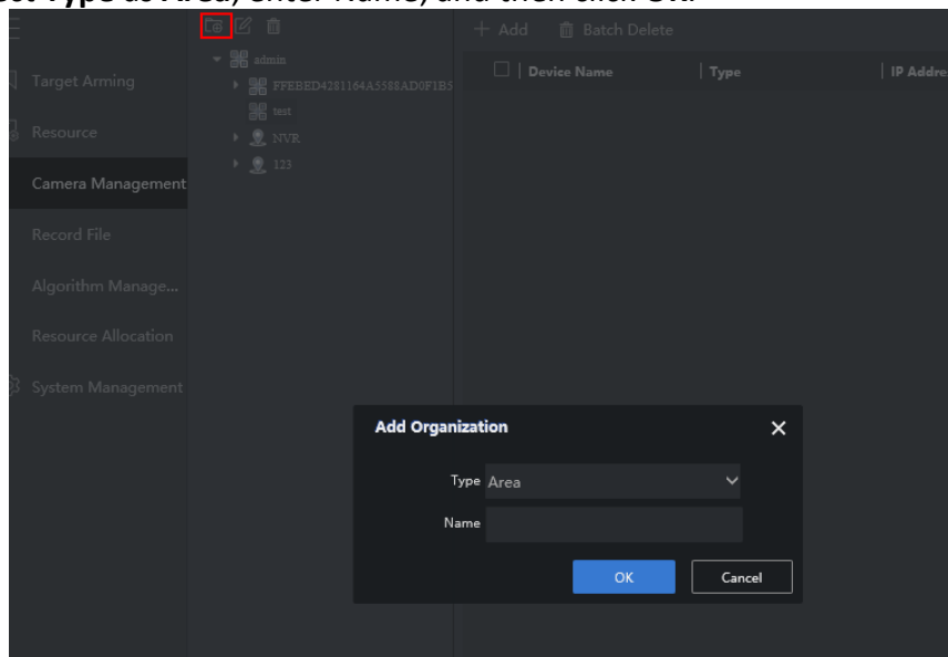
Figure 3-6 Add Area
