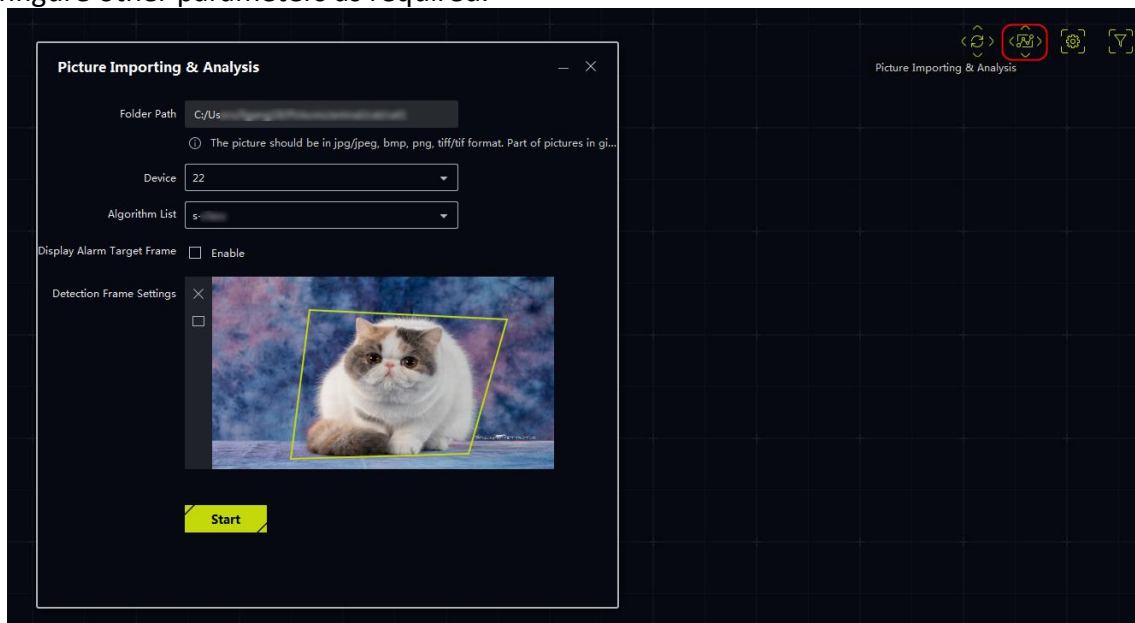
Figure 3-27 Import Picture
