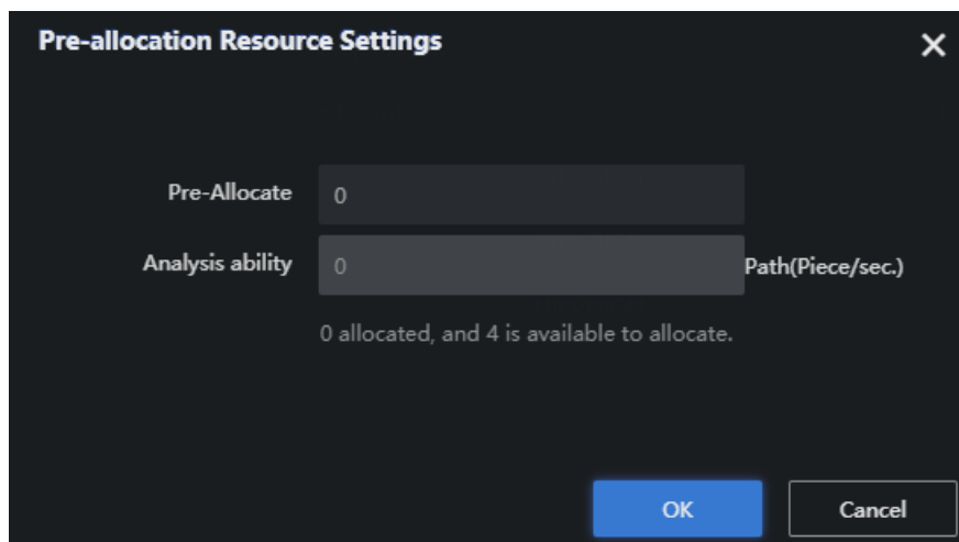
Figure 3-3 Pre-allocation Resource
