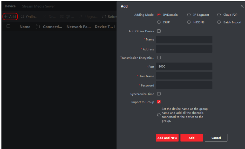
Figure 3-24 Add Server
