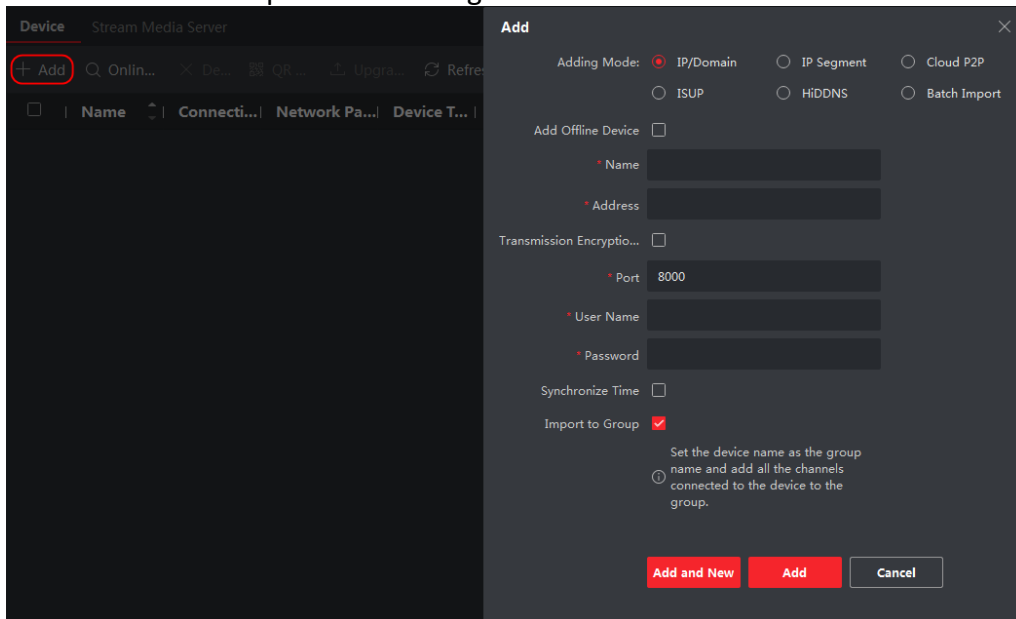
Figure 3-30 Add Server
