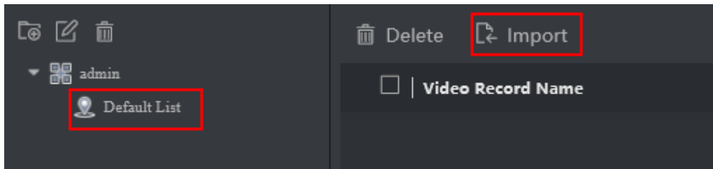
Figure 3-9 Import File
