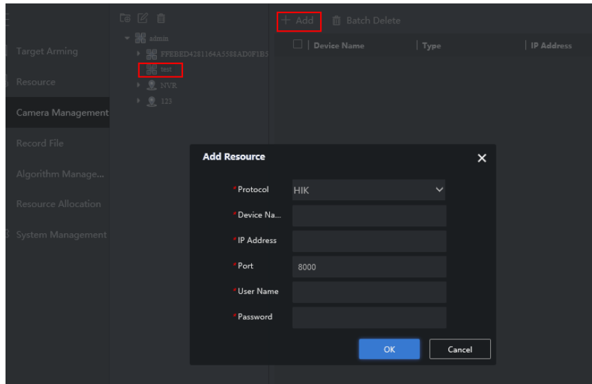
Figure 3-5 Add Camera
