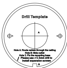
Figure 2-3 Drill Template
