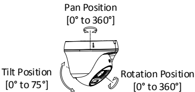
Figure 2-6 3-Axis Adjustment
