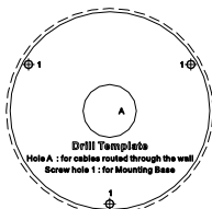
Figure 2-26 Drill Template
