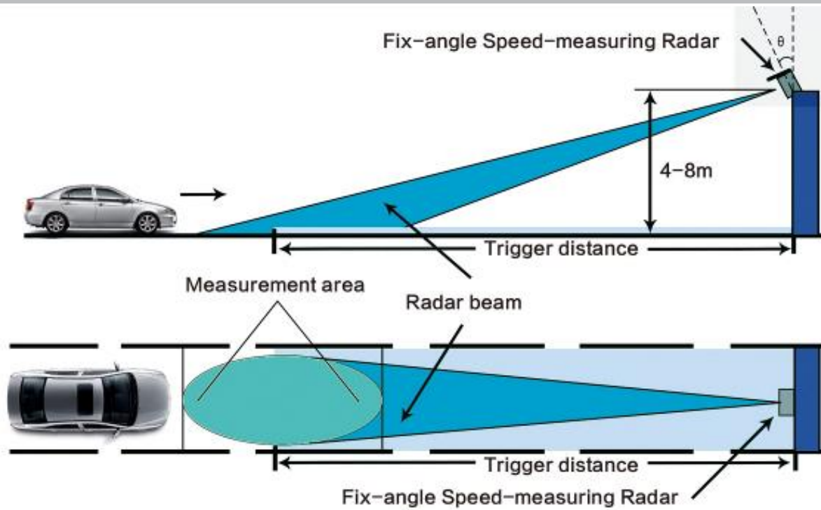
Application diagram
