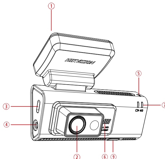
Figure 1, Left View
