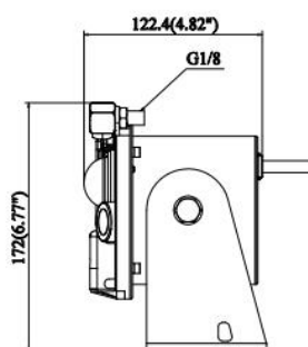
Camera dimensions
