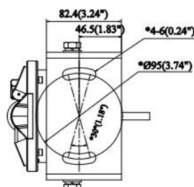
Bracket dimensions (* indicates mounting hole dimensions)
