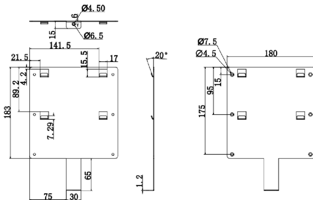
Wall Mounted Bracket
