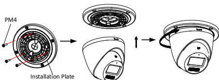
Figure 2-8 Fix the Camera to the Junction Box Cover
