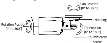
Figure 2-2 3-Axis Adjustment
