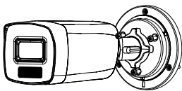
Figure 2-3 Fix the Camera to the Junction Box Cover
