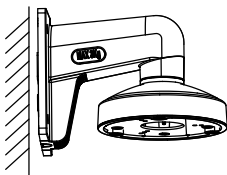
Figure 2-10 Fix the Wall Mount
