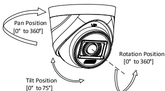
Figure 2-19 3-Axis Adjustment
