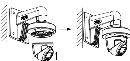
Figure 2-15 Finish Installation
