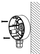
Figure 2-4 Secure Junction Box on Wall
