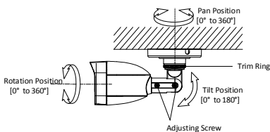
Figure 2-2 3-Axis Adjustment
