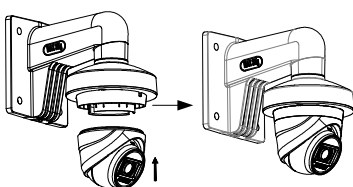
Figure 2-26 Finish Installation
