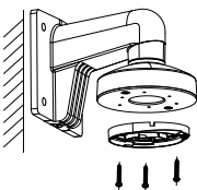
Figure 2-14 Fix Base
