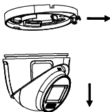
Figure 2-6 Disassemble Camera
