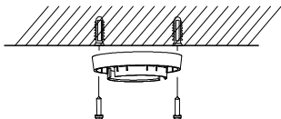
Figure 2-17 Secure Base to Ceiling
