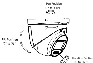
Figure 2-8 3-Axis Adjustment
