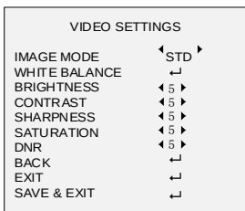
Figure 4-3 VIDEO SETTINGS
