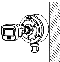
Figure 2-5 Fix Cover to Its Body
