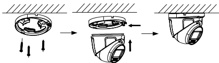
Figure 2-7 Install Camera to Ceiling
