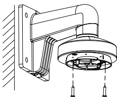
Figure 2-25 Fix the Base onto Wall Mount
