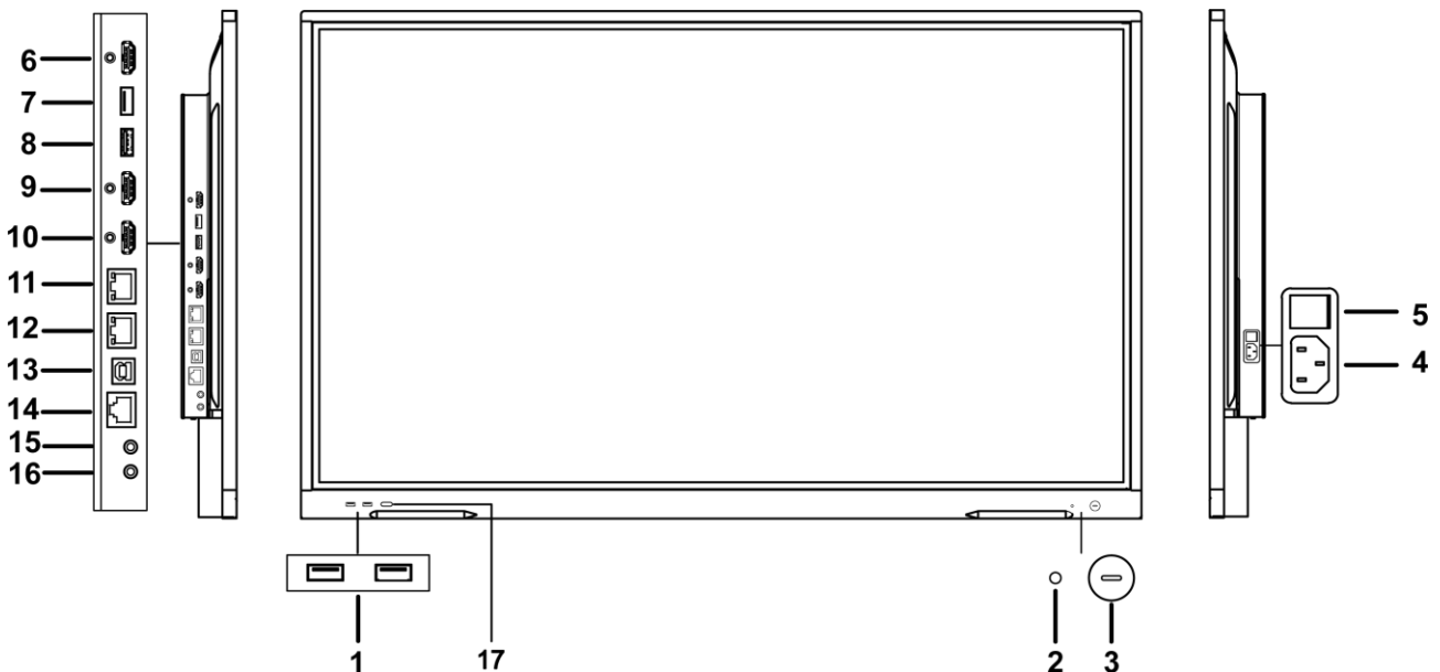
Figure 3-1 Front Panel and Interfaces
