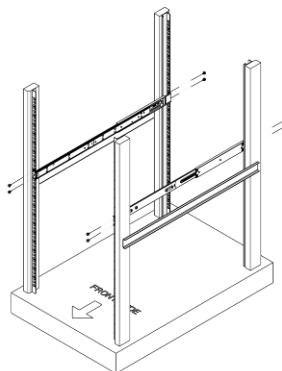
② Install Outer Rails
