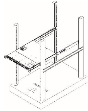
③ Install Server into Rack
