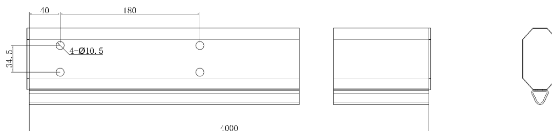
4 m octagonal boom pole
