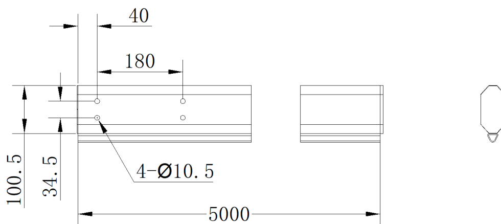
5m octagonal pole
