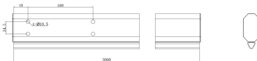
3 m octagonal boom pole
