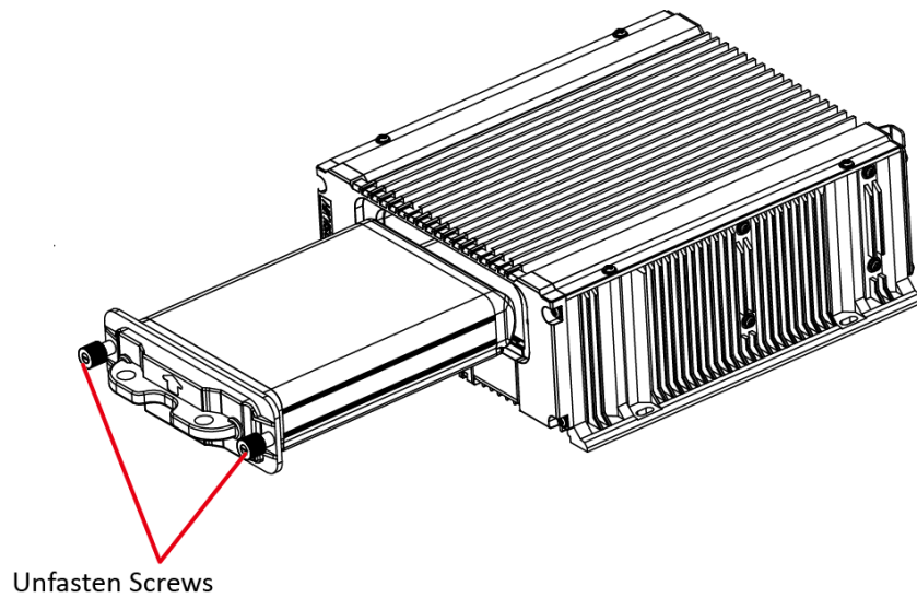
Figure 2-19 Unfasten Screws
