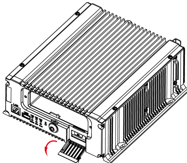
Figure 2-20 Open Cover
