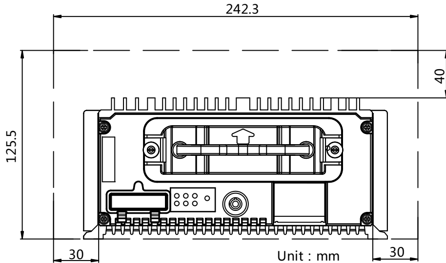
Figure 2-1 Recommended Installation Space
