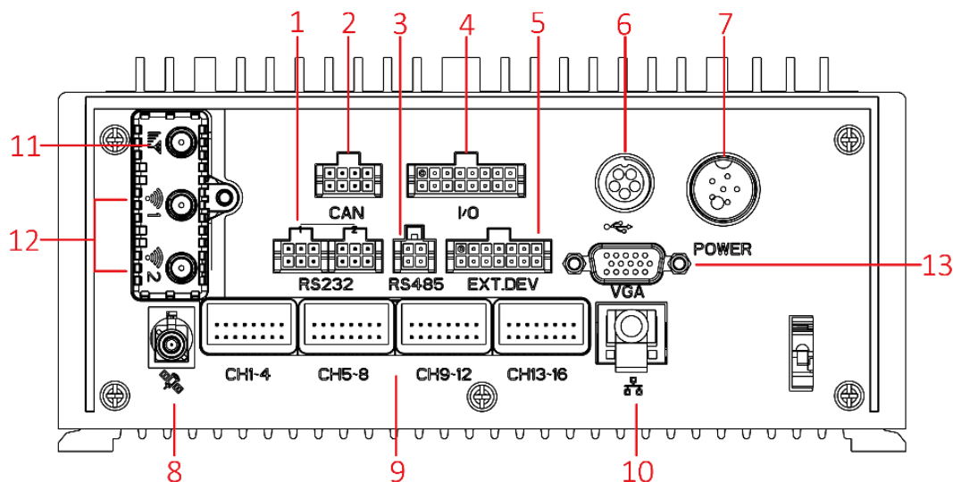
Figure 1-2 Front Panel
