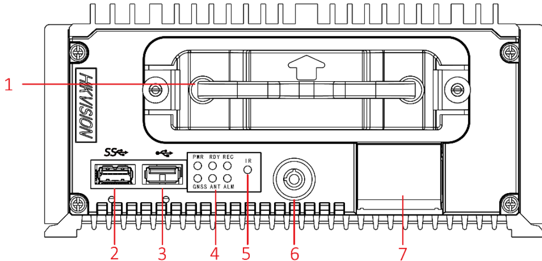
Figure 1-1 Front Panel
