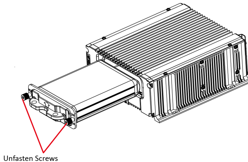
Figure 2-4 Pull Dummy HDD out
